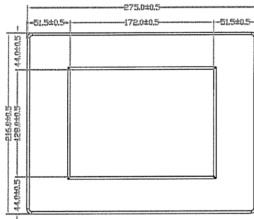
New Front Bezel Dimension:
