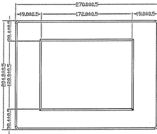
Original Front Bezel Dimension:
